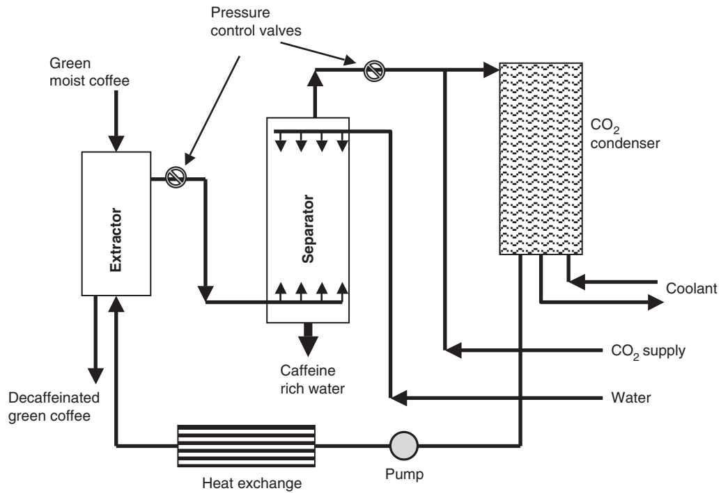
Figure 9.24 Layout of SCF CO 2 extraction for decaffeination process. (Redrawn from McHugh and Krukoni (1994), Supercritical Fluid Extraction: Principles and Practice , 2nd edn. Butterworth-Heinemann, Boston.)
