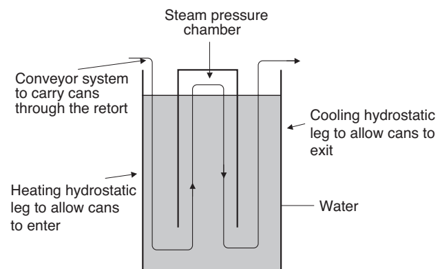
Figure 9.33 Hydrostatic retort.
