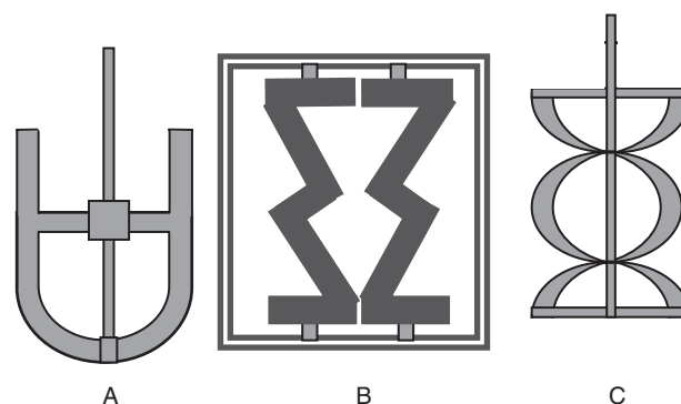
Figure 9.28 Devices for the mixing of high-viscosity fluids: A an anchor impeller; B a double z-blade mixer; C a double-flight helical-ribbon impeller.
