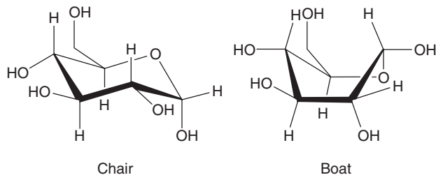
Figure 2.4 Chair and boat conformations of α-D-glucopyranose.
