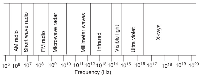
Figure 8.3 Spectrum of electromagnetic radiation.
