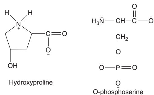
Figure 2.11 Chemical structures of some non-standard amino acids common in food proteins.
