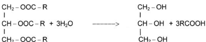
FIGURE 12.8 Hydrolytic rancidity.
