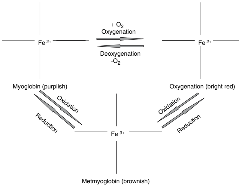
FIGURE 9.4 Pigment change.
