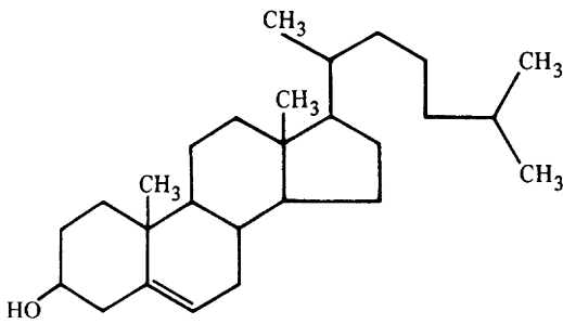
FIGURE 12.4 Cholesterol, phytosterols.
