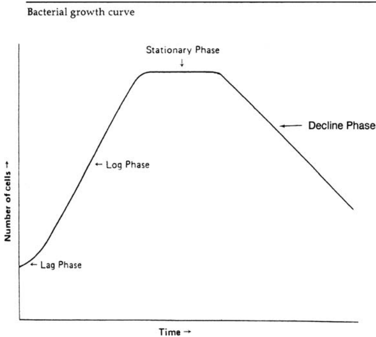
FIGURE 16.1 Bacterial growth curve
