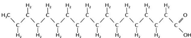
FIGURE 12.5 Example of a fatty acid.
