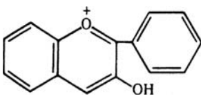
FIGURE 7.4 Anthocyanin.
